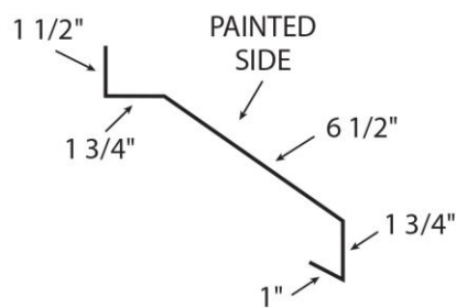
TRACK COVER
