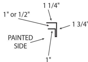
F TRIM
