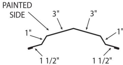
RIDGE CAP
