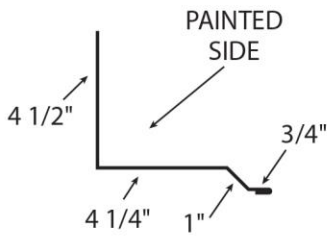
SIDE WALL
