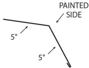
UPPER GAMBREL
