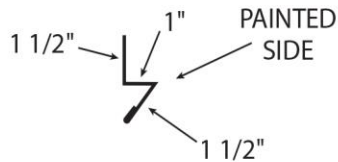
RAT GUARD
