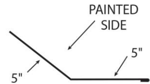
ROOF TRANSITION
