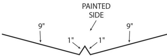
RESIDENTIAL VALLEY
