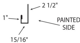
J TRIM
