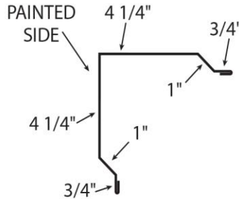
J TRIM
