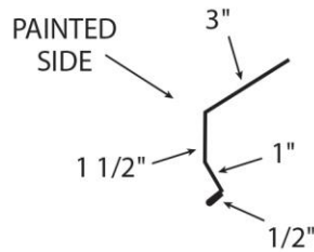
RE-DRIP
