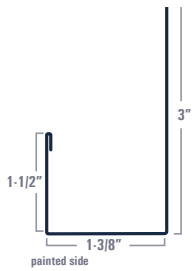
J Trim
