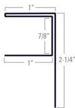
F Trim for Panel
