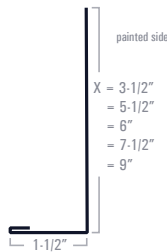
Fascia
