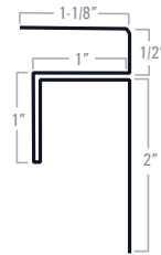
F&J for Soffit
