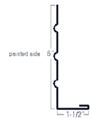
CUSTOM TRIM
