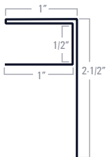
F Trim for Soffit
