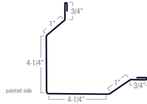
Outside Rake Corner
