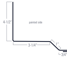
Sidewall
