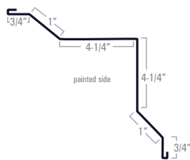
Inside Corner
