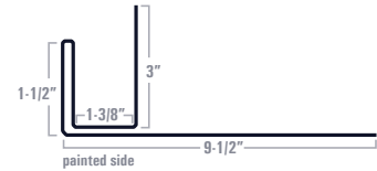
Overhead Door Trim
