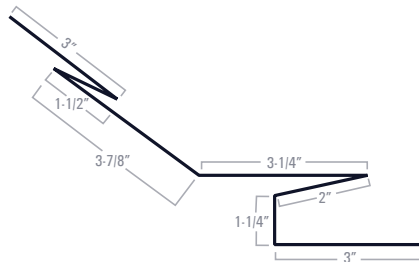
Box Style Endwall
