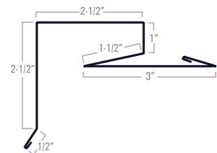
Box Style Residential Rake
